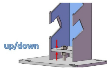
Patented clamping device
